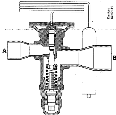
Balanced port design Adjustable setting
